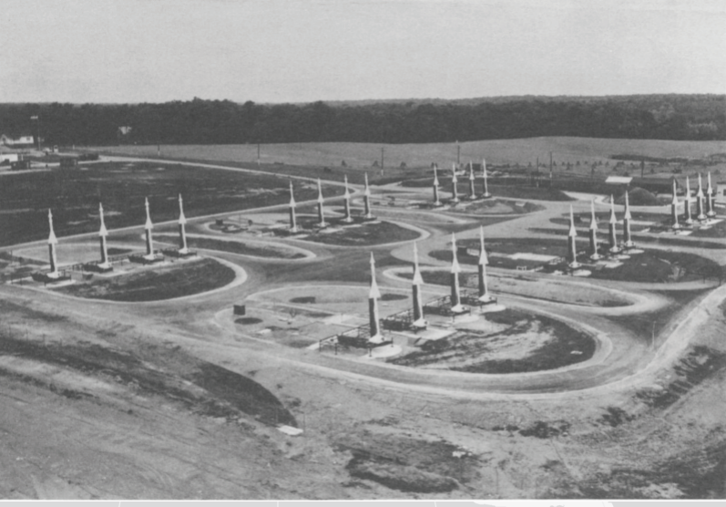
The control site (above) and launch site (below) of Nike Missile Defense Site W-64, located in Lorton, VA. W-64 was the first fixed Nike site in the U.S. It was a double site, meaning it housed six Nike magazines (seen below) as opposed to the standard three. Images courtesy of Christopher Bright, "Nike Defends Washington: Antiaircraft Missiles in Fairfax County, VA During the Cold War, 1954-1974".
